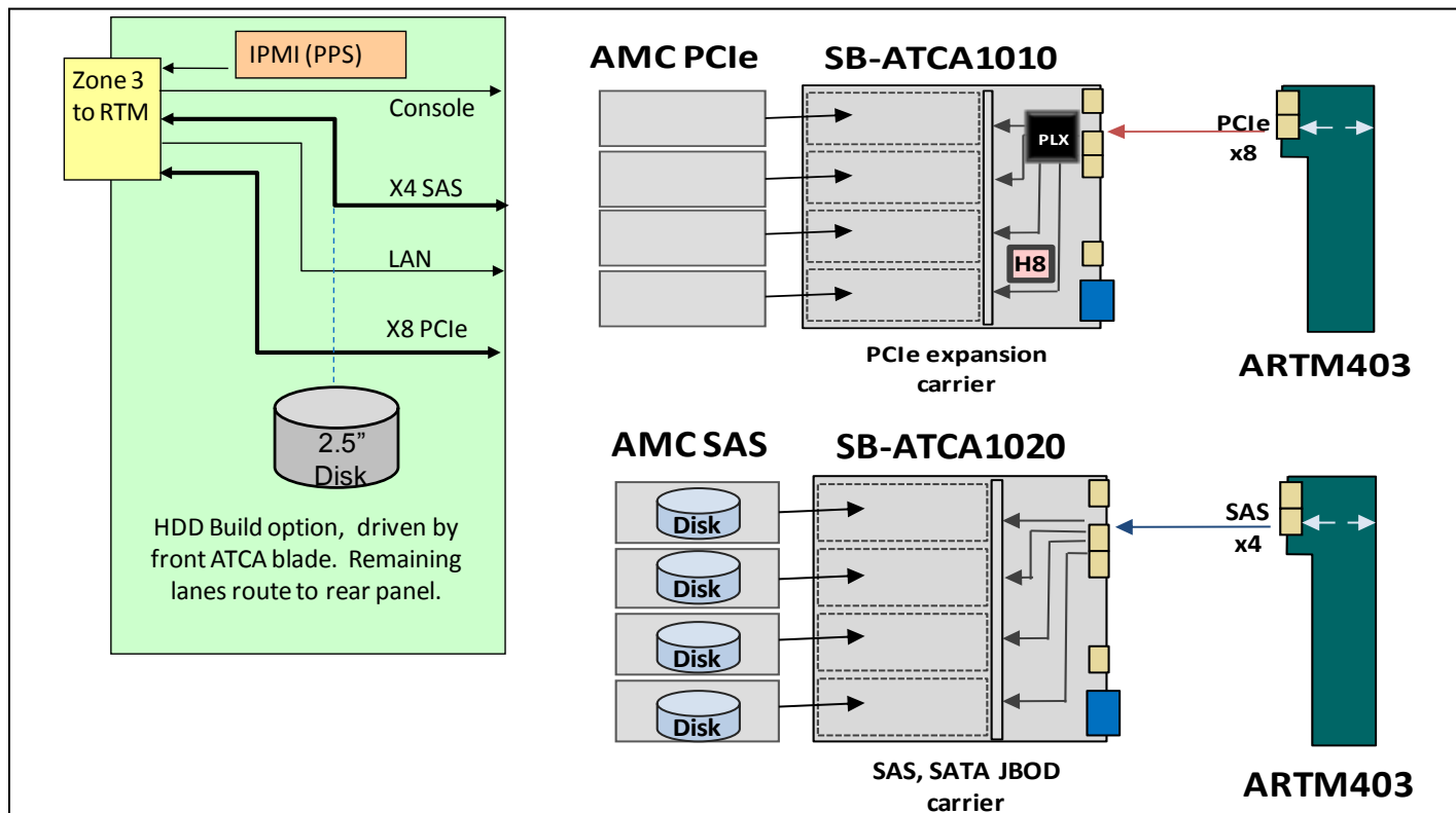
ARTM403 Block Diagram and Deployment Concept
