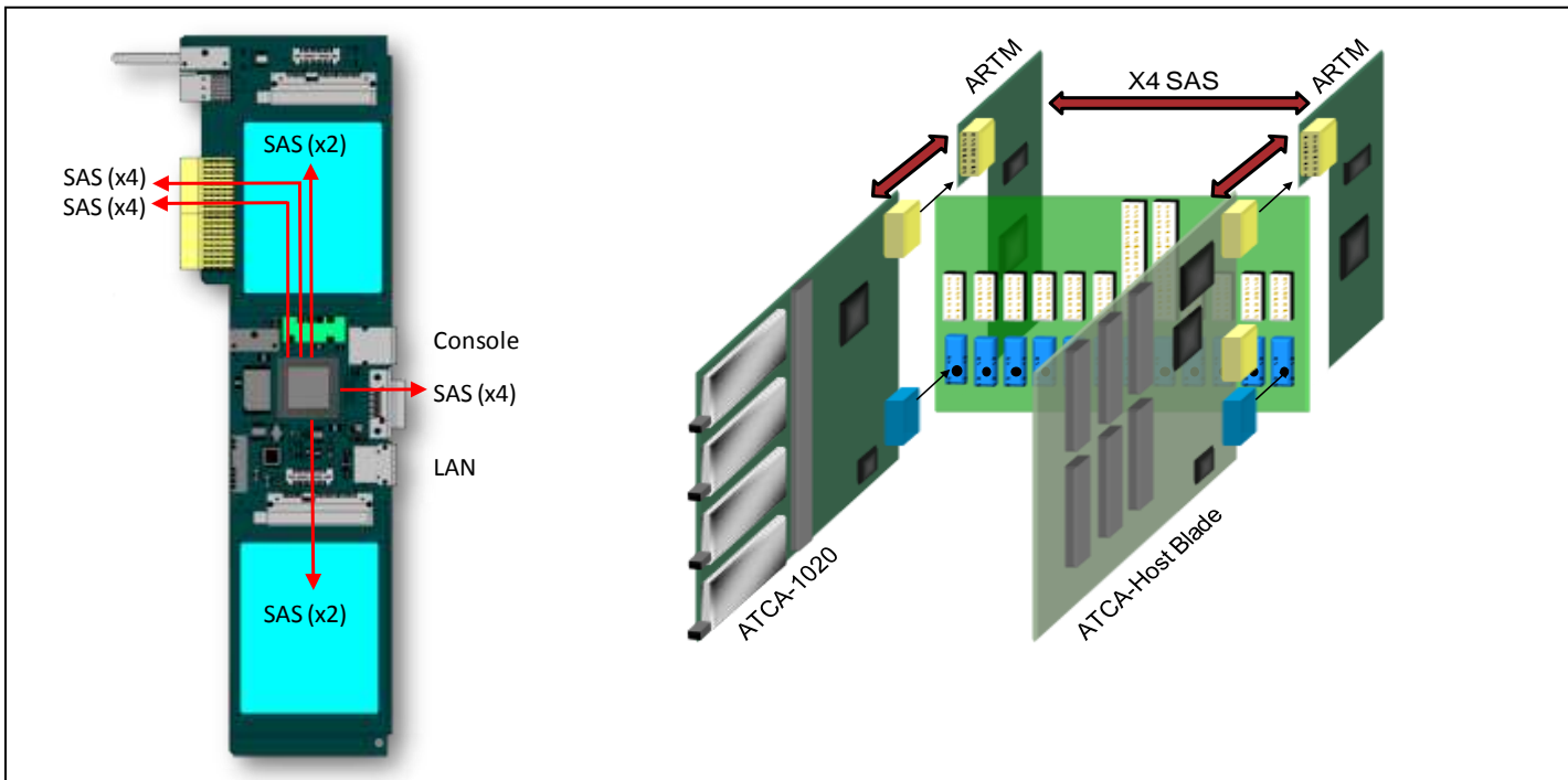
RTM401 Block Diagram and Deployment Concept
