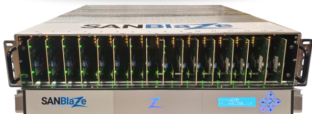
SANBlaze SBExpress-RM6 Gen6 PCIe NVMe SSD Test System
